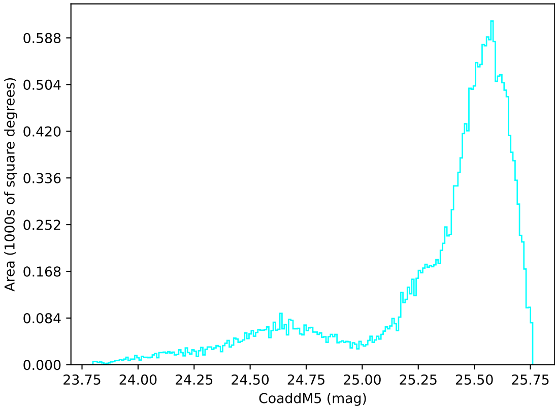
internal_u_expt27_nscale1.5v3.4_10yrs All sky u band: CoaddM5
