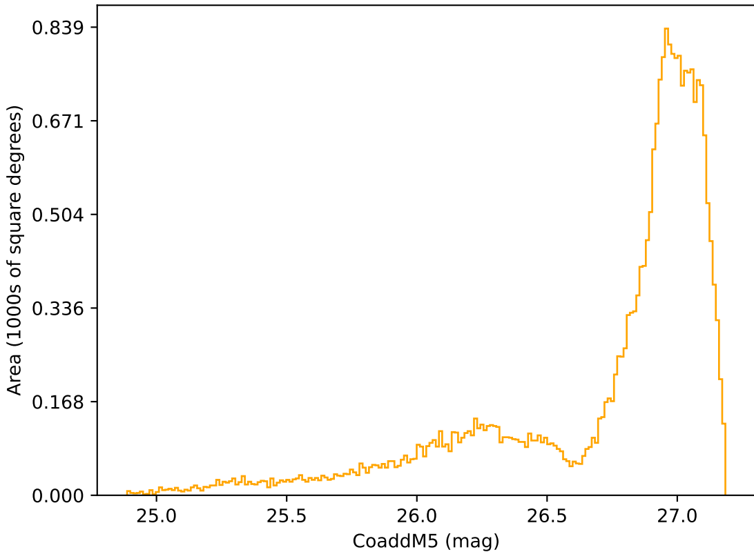
internal_u_expt27_nscale1.5v3.4_10yrs All sky r band: CoaddM5
