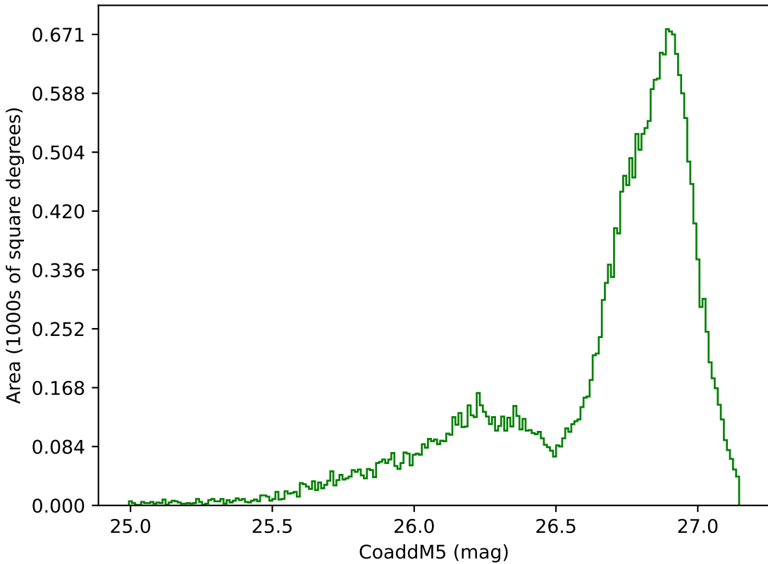
internal_u_expt27_nscale1.5v3.4_10yrs All sky g band: CoaddM5
