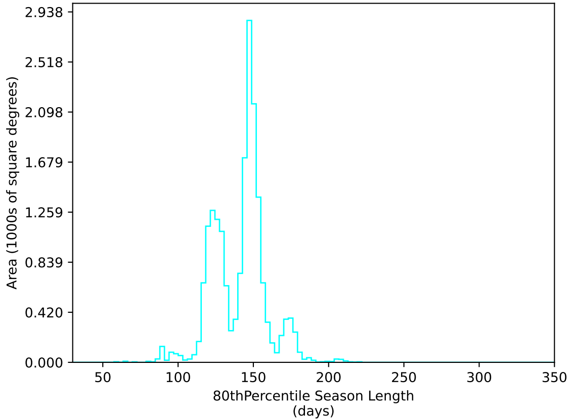
internal_u_expt27_nscale1.5v3.4_10yrs WFD u band: 80thPercentile Season Length
