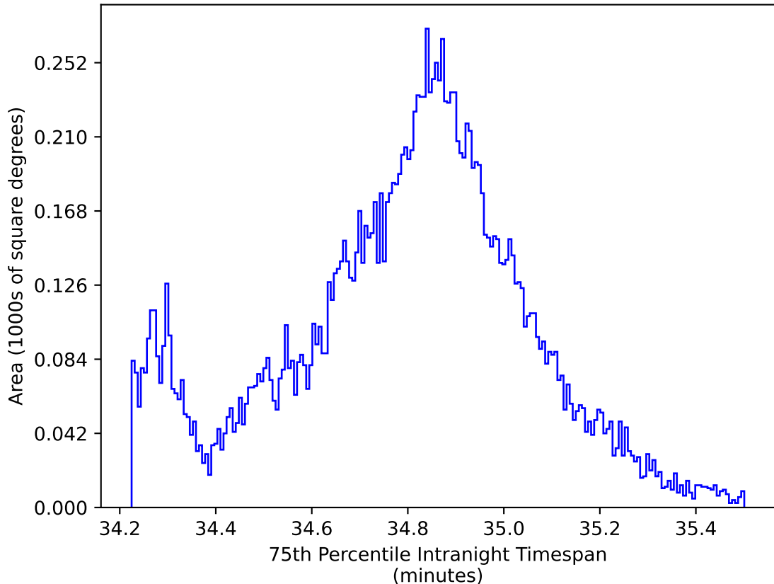
internal_u_expt27_nscale1.5v3.4_10yrs WFD all bands: 75th Percentile Intranight Timespan
