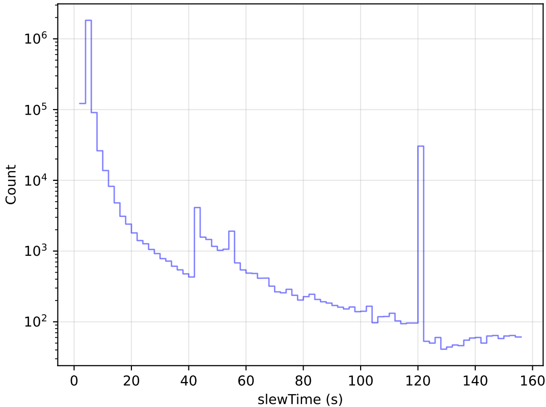
internal_u_expt27_nscale1.5v3.4_10yrs All visits: Slew Time Histogram
