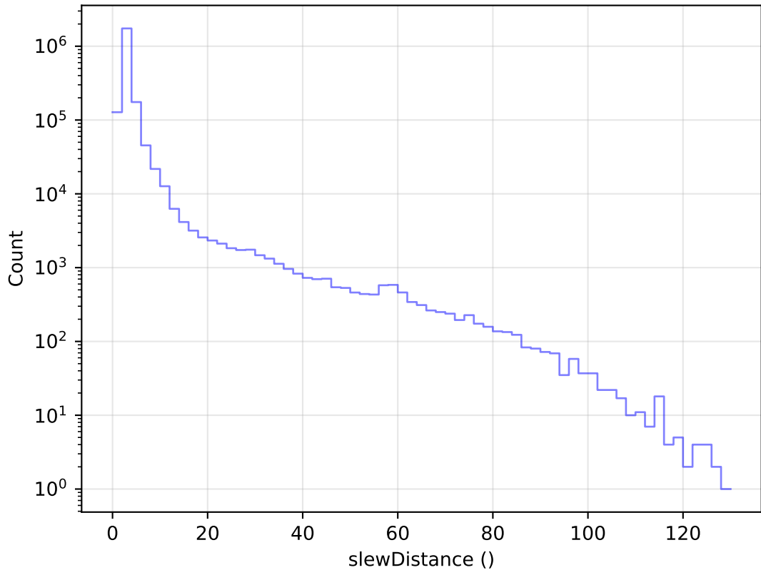
internal_u_expt27_nscale1.5v3.4_10yrs All visits: Slew Distance Histogram
