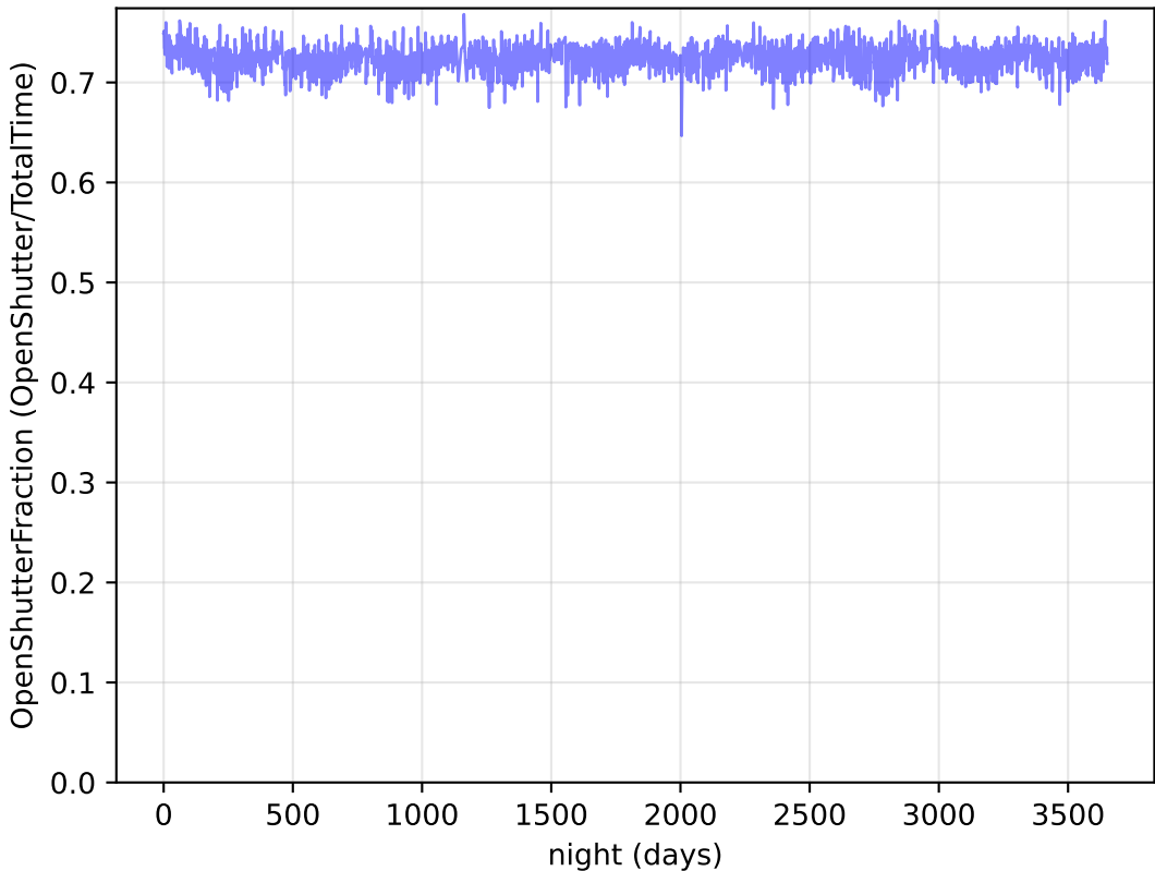
internal_u_expt27_nscale1.5v3.4_10yrs : OpenShutterFraction
