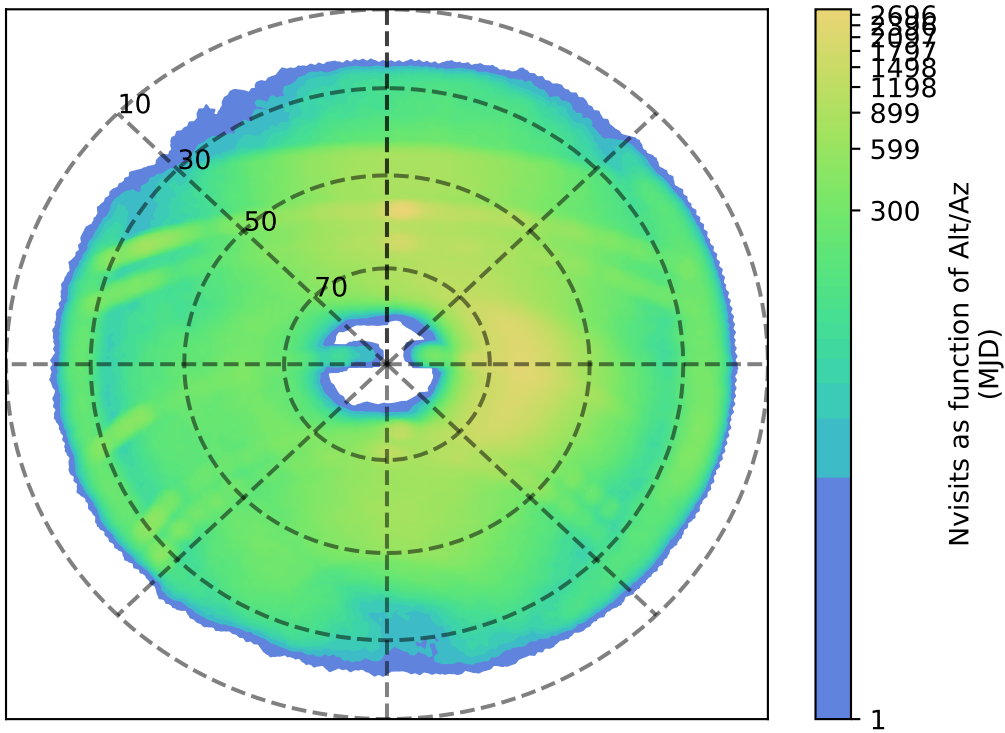
internal_u_expt27_nscale1.5v3.4_10yrs i: Nvisits as function of Alt/Az
