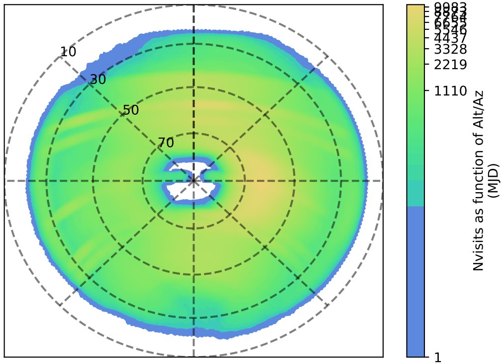
internal_u_expt27_nscale1.5v3.4_10yrs : Nvisits as function of Alt/Az
