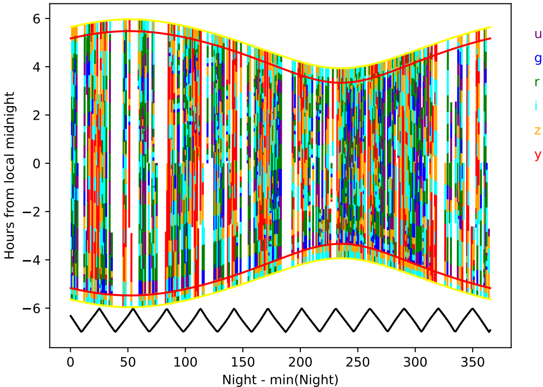
internal_u_expt27_nscale1.5v3.4_10yrs year 7-8: Hourglass
