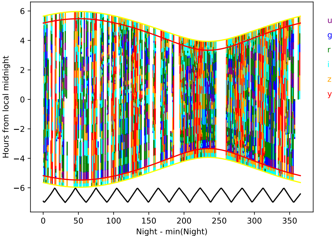
internal_u_expt27_nscale1.5v3.4_10yrs year 5-6: Hourglass
