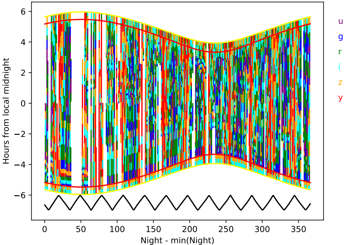
internal_u_expt27_nscale1.5v3.4_10yrs year 2-3: Hourglass
