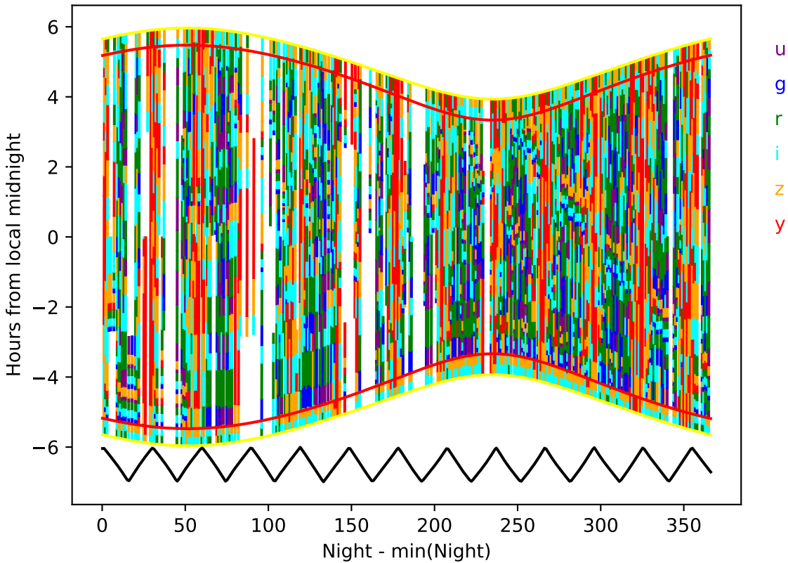
internal_u_expt27_nscale1.5v3.4_10yrs year 1-2: Hourglass
