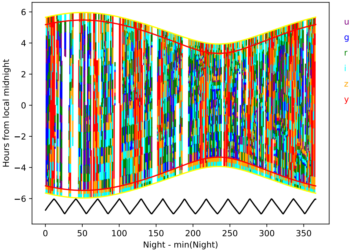
internal_u_expt27_nscale1.5v3.4_10yrs year 0-1: Hourglass
