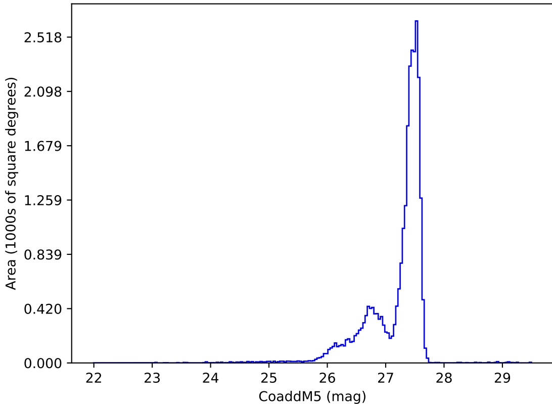
internal_u_expt27_nscale1.5v3.4_10yrs : CoaddM5
