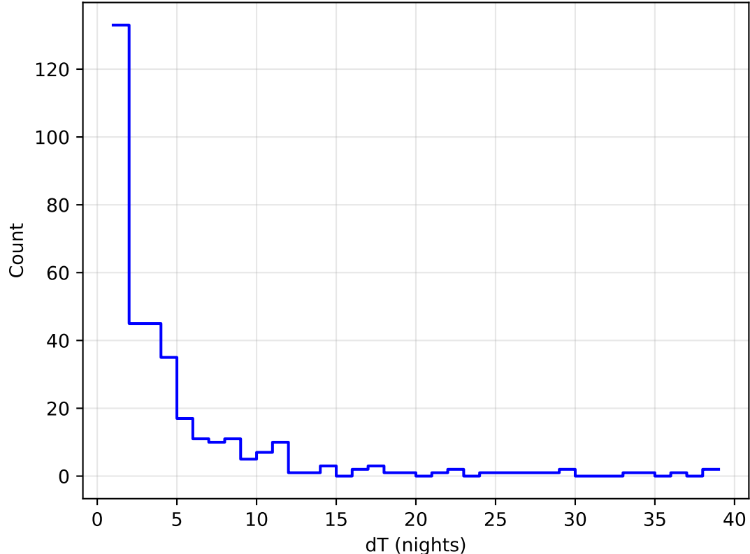
internal_u_expt27_nscale1.5v3.4_10yrs all bands: DD:WFD Delta Nights Histogram
