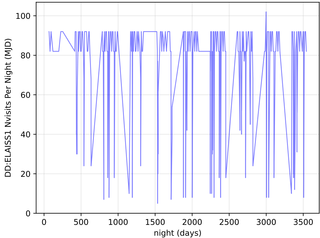
internal_u_expt27_nscale1.5v3.4_10yrs all bands: DD:ELAISS1 Nvisits Per Night
