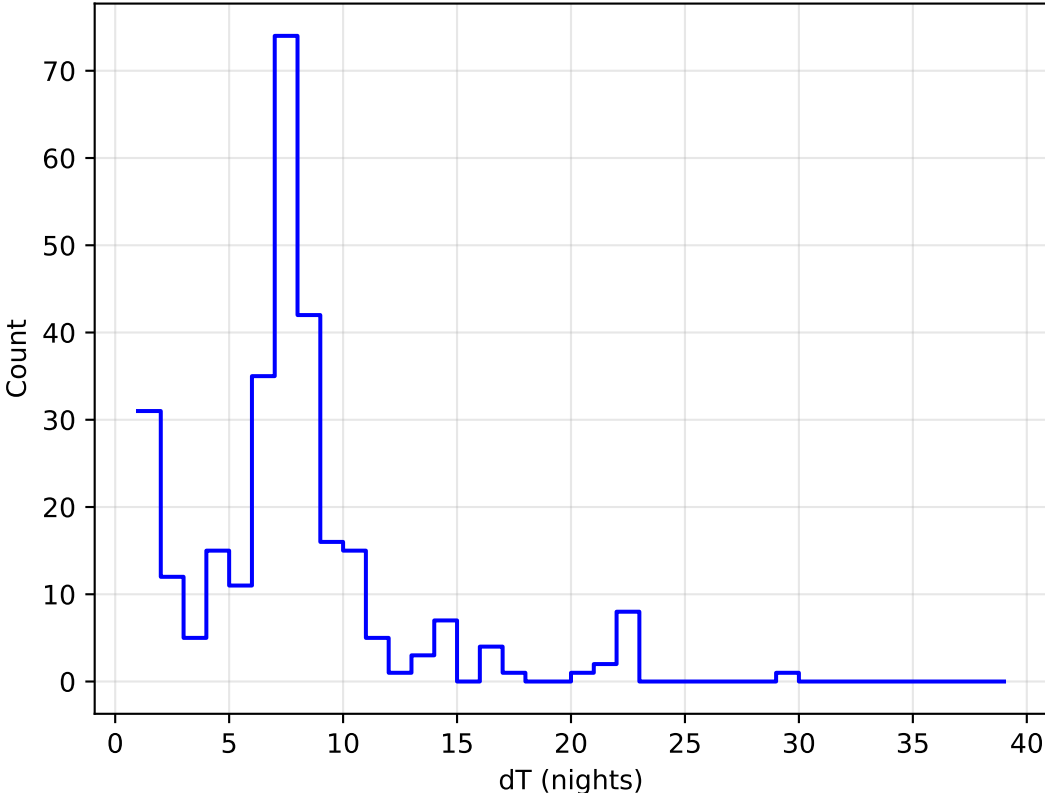
internal_u_expt27_nscale1.5v3.4_10yrs all bands: DD:EDFS Delta Nights Histogram
