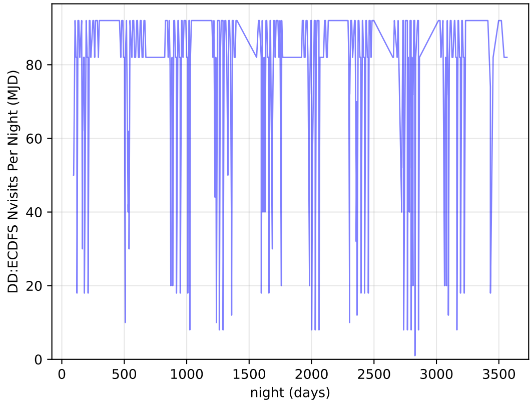
internal_u_expt27_nscale1.5v3.4_10yrs all bands: DD:ECDFS Nvisits Per Night
