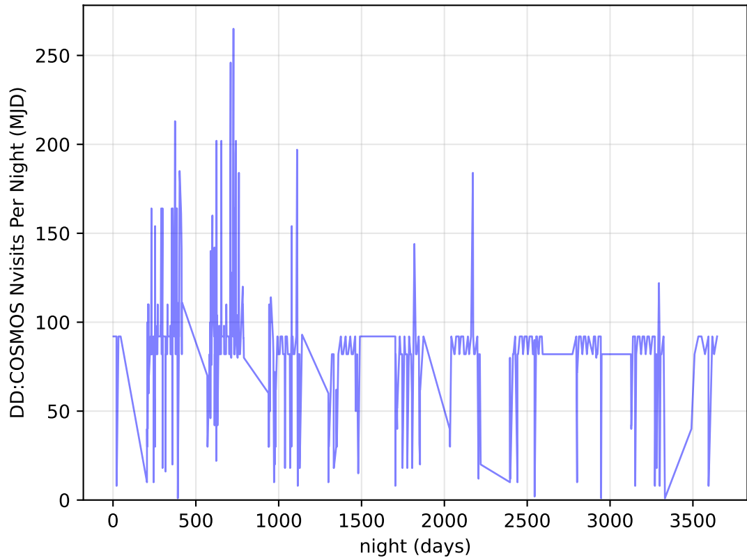
internal_u_expt27_nscale1.5v3.4_10yrs all bands: DD: COSMOS Nvisits Per Night
