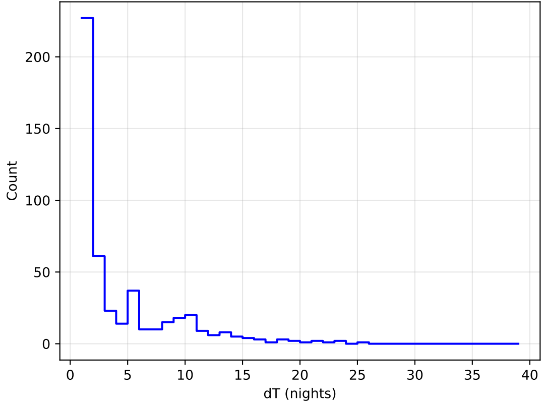
internal_u_expt27_nscale1.5v3.4_10yrs all bands: DD:COSMOS Delta Nights Histogram
