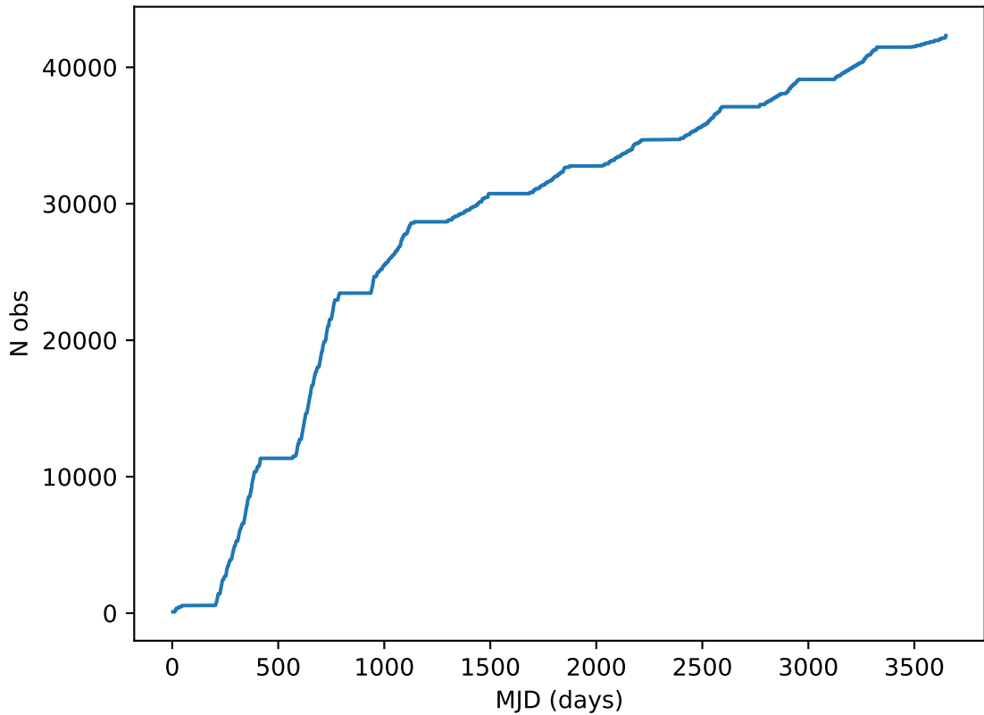
internal_u_expt27_nscale1.5v3.4_10yrs all bands: DD: COSMOS Cumulative NVisits
