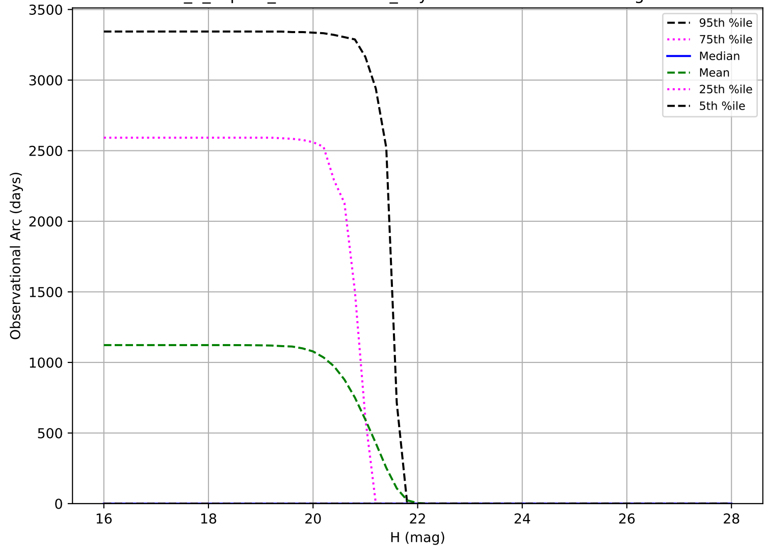
internal_u_expt27_nscale1.2v3.4_10yrs: Observational Arc Length Vatra
