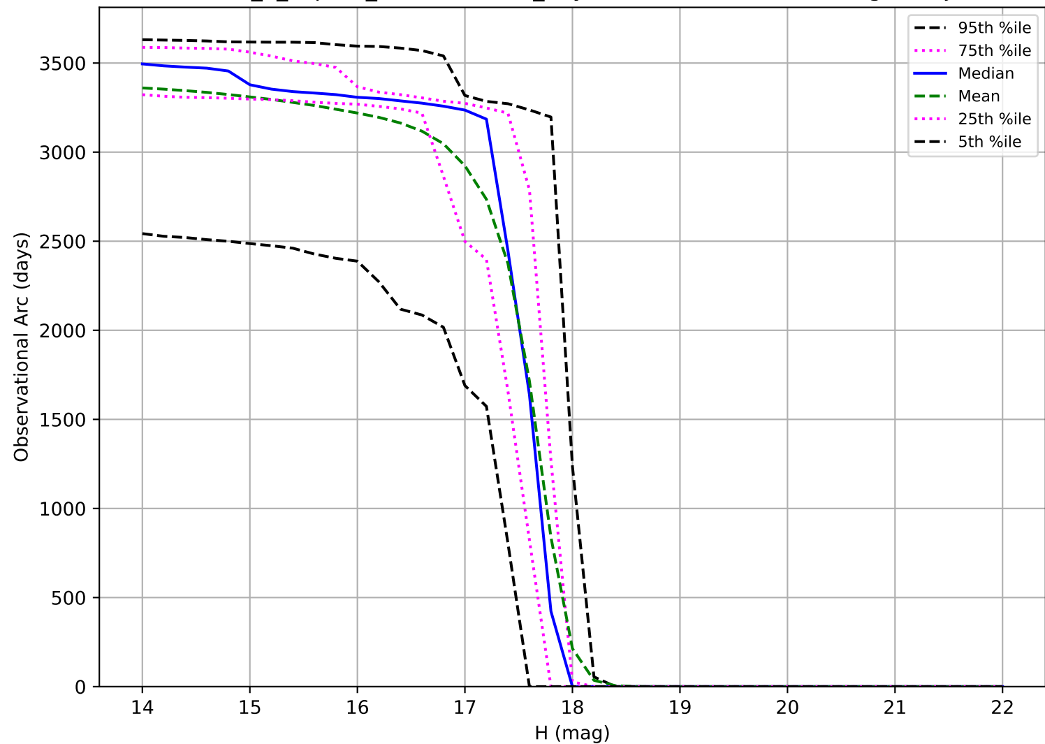
internal_u_expt27_nscale1.2v3.4_10yrs: Observational Arc Length Trojan
