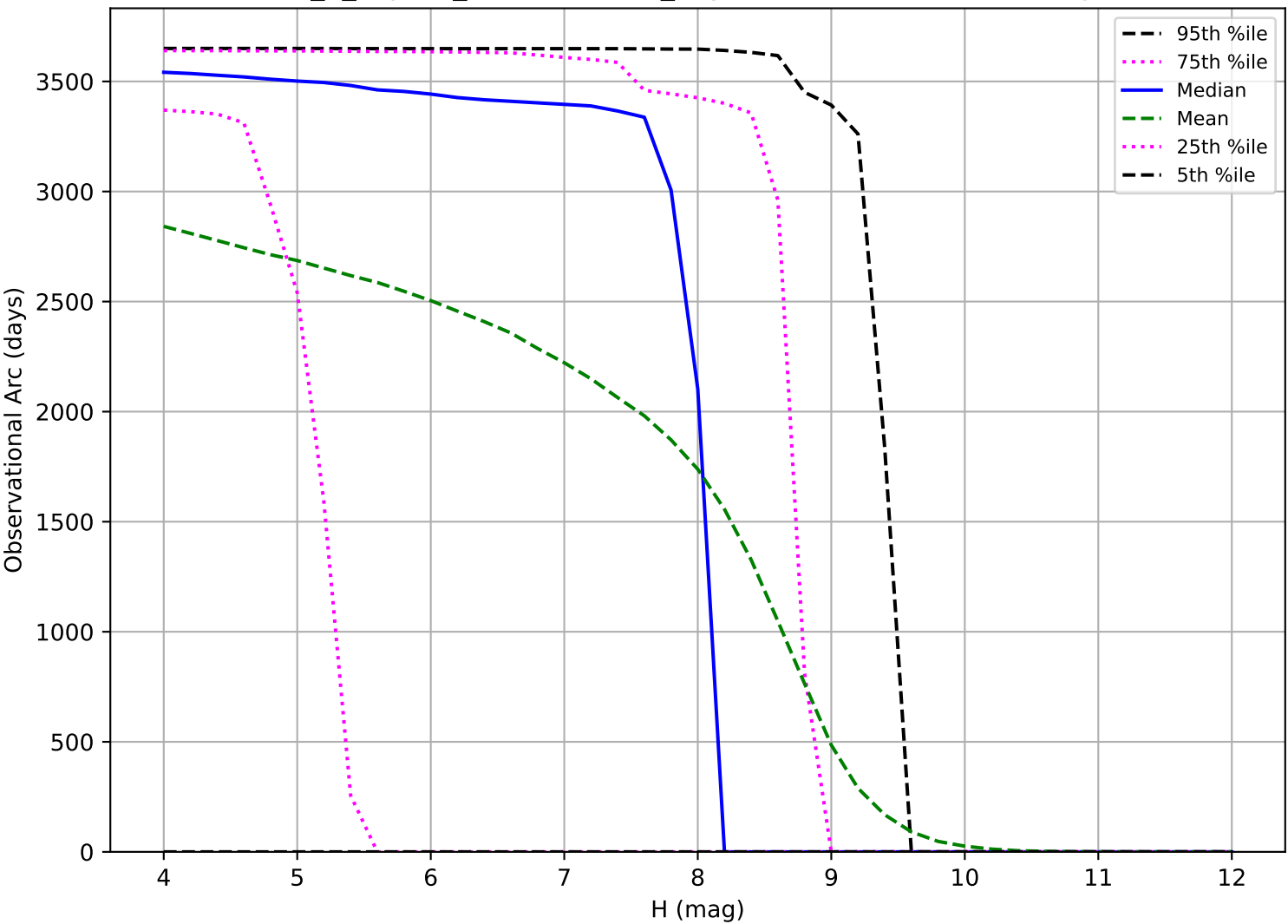
internal_u_expt27_nscale1.2v3.4_10yrs: Observational Arc Length TNO
