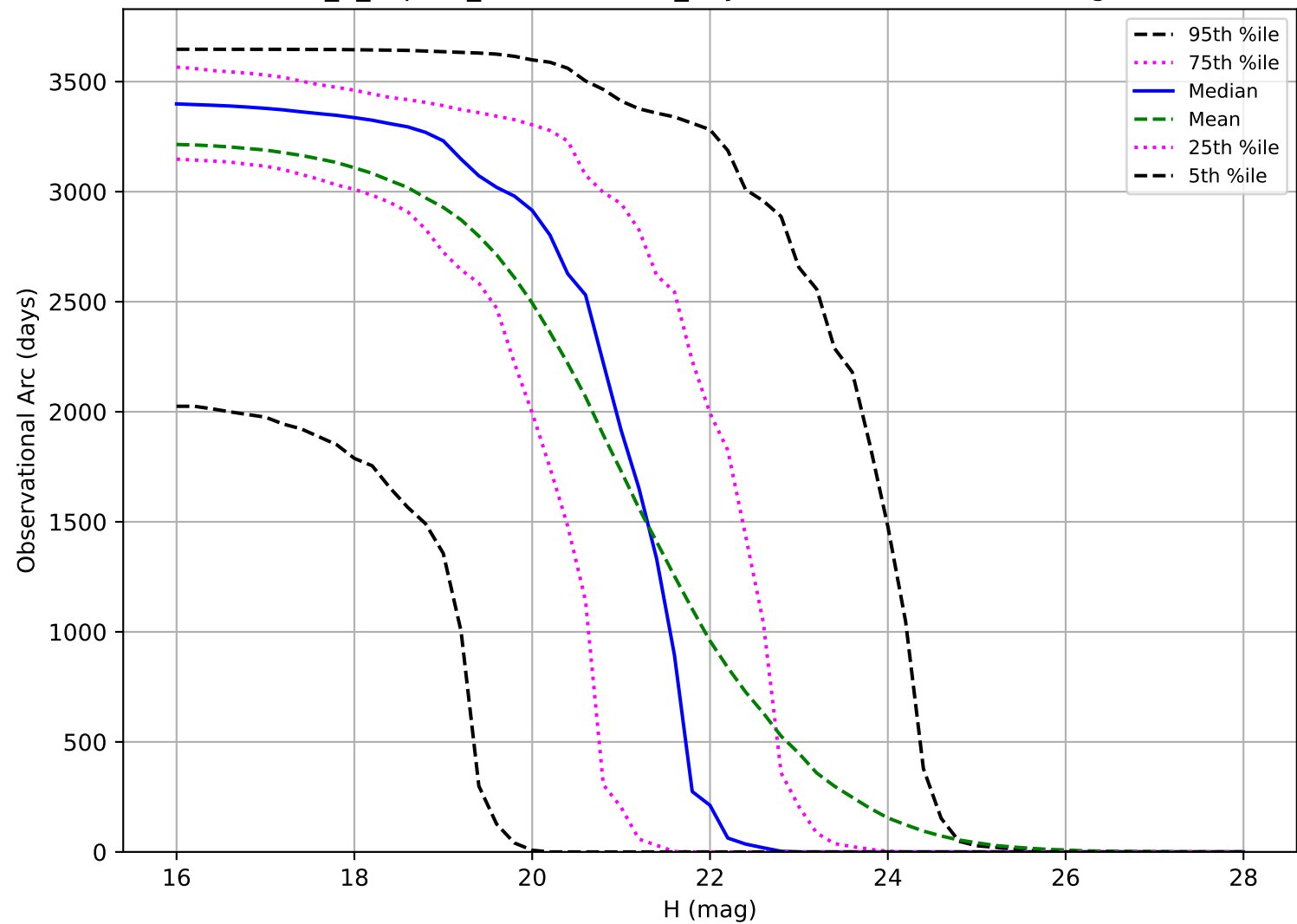
internal_u_expt27_nscale1.2v3.4_10yrs: Observational Arc Length PHA
