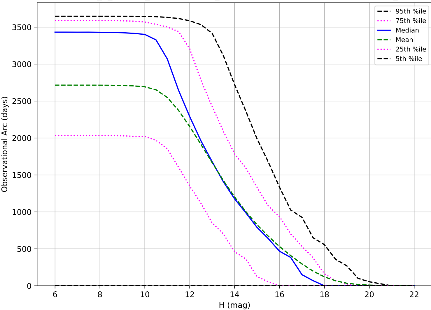
internal_u_expt27_nscale1.2v3.4_10yrs: Observational Arc Length OCC_r5
