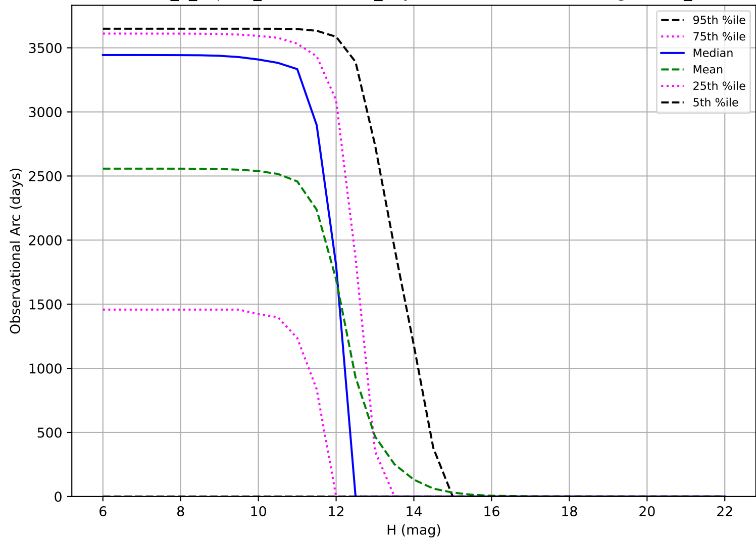
internal_u_expt27_nscale1.2v3.4_10yrs: Observational Arc Length OCC_r20
