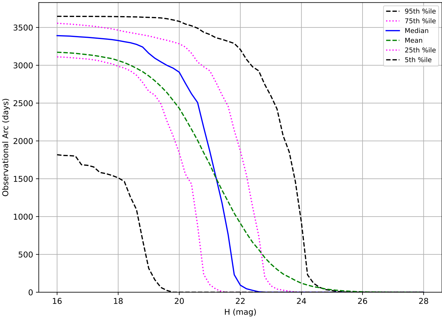
internal_u_expt27_nscales1.2v3.4_10yrs: Observational Arc Length NEO
