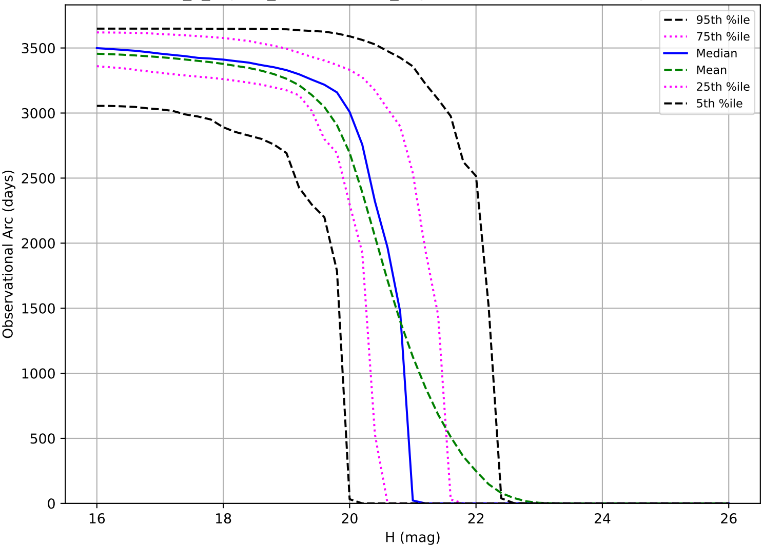
internal_u_expt27_nscale1.2v3.4_10yrs: Observational Arc Length MBA
