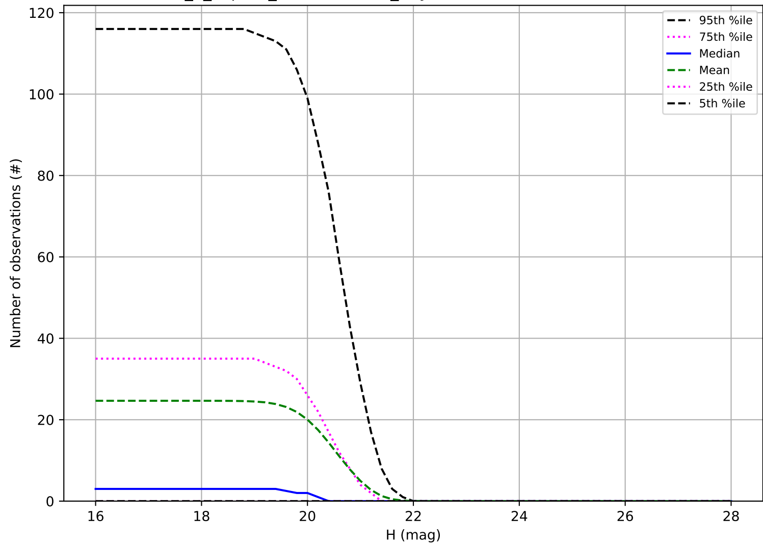
internal_u_expt27_nscale1.2v3.4_10yrs: Number of observations Vatira
