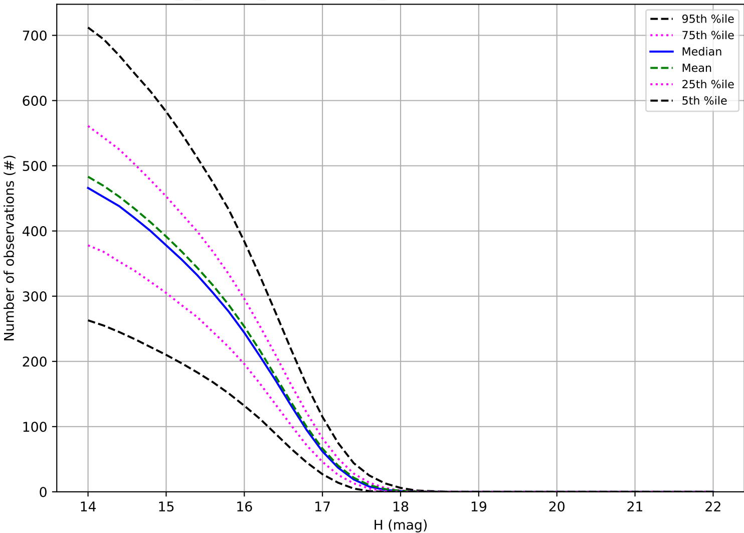
internal_u_expt27_nscale1.2v3.4_10yrs: Number of observations Trojan
