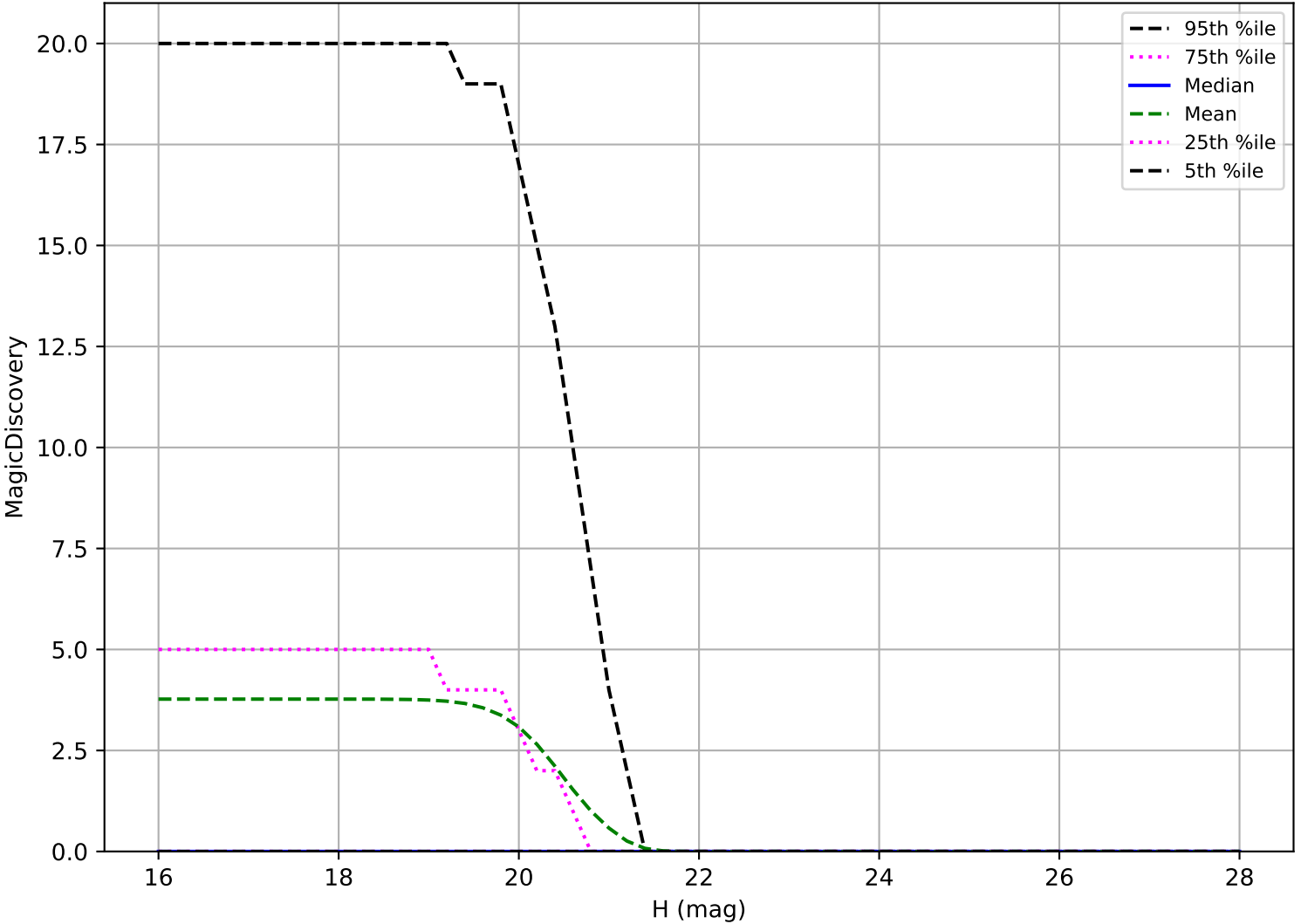
internal_u_expt27_nscale1.2v3.4_10yrs: Vatira 6 detections in 60 nights detection loss
