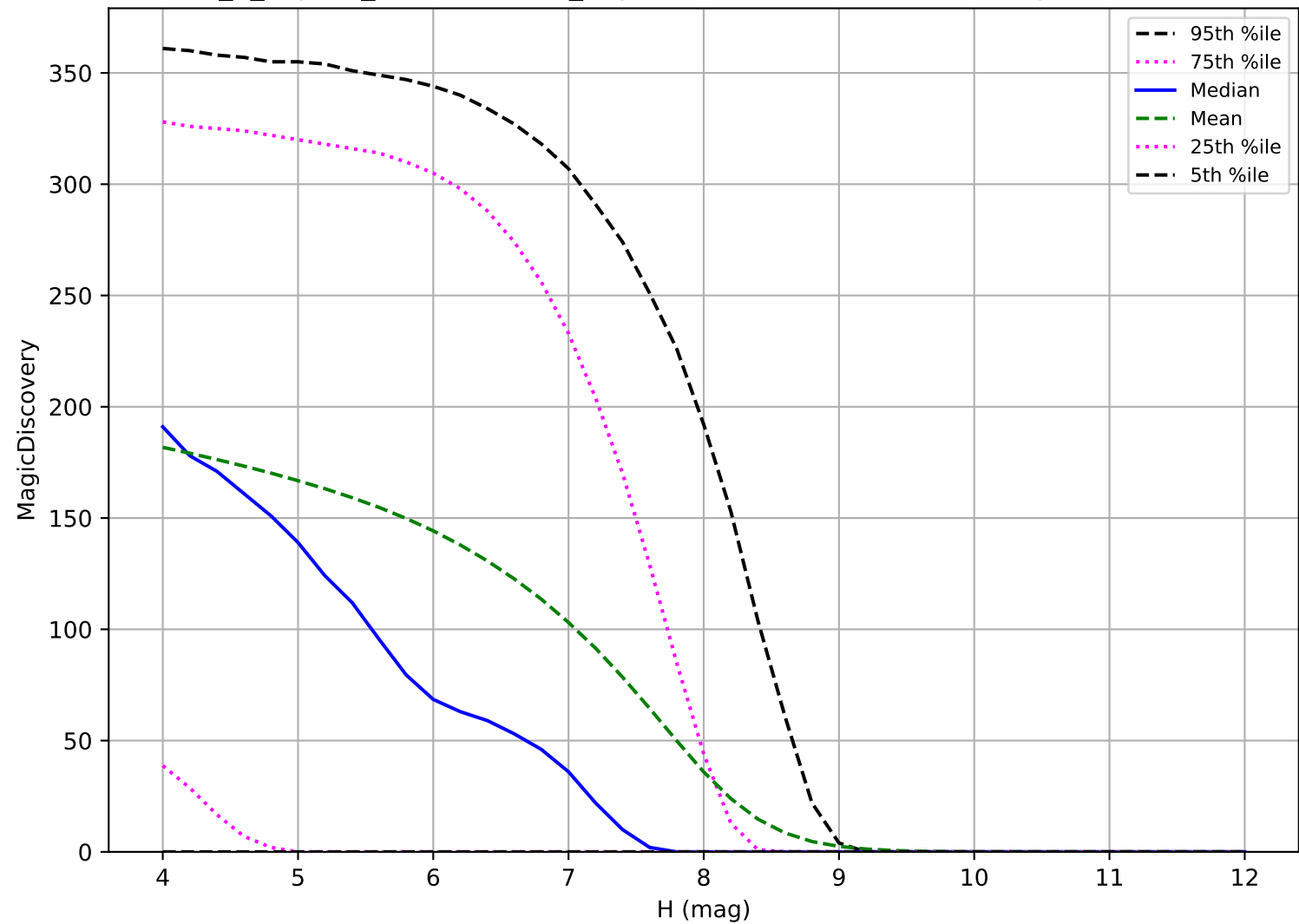
internal_u_expt27_nscale1.2v3.4_10yrs: TNO 6 detections in 60 nights detection loss
