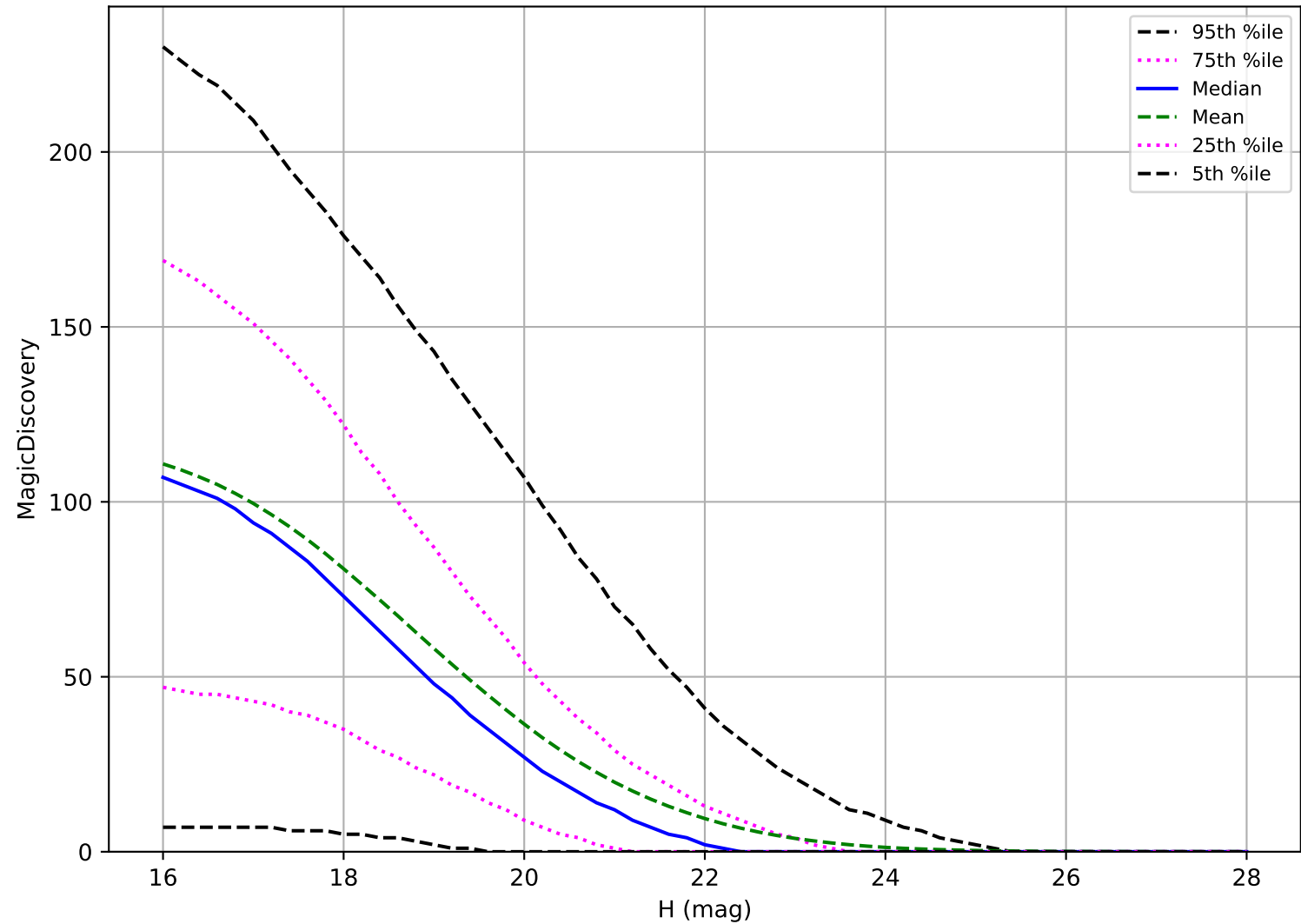
internal_u_expt27_nscale1.2v3.4_10yrs: PHA 6 detections in 60 nights detection loss
