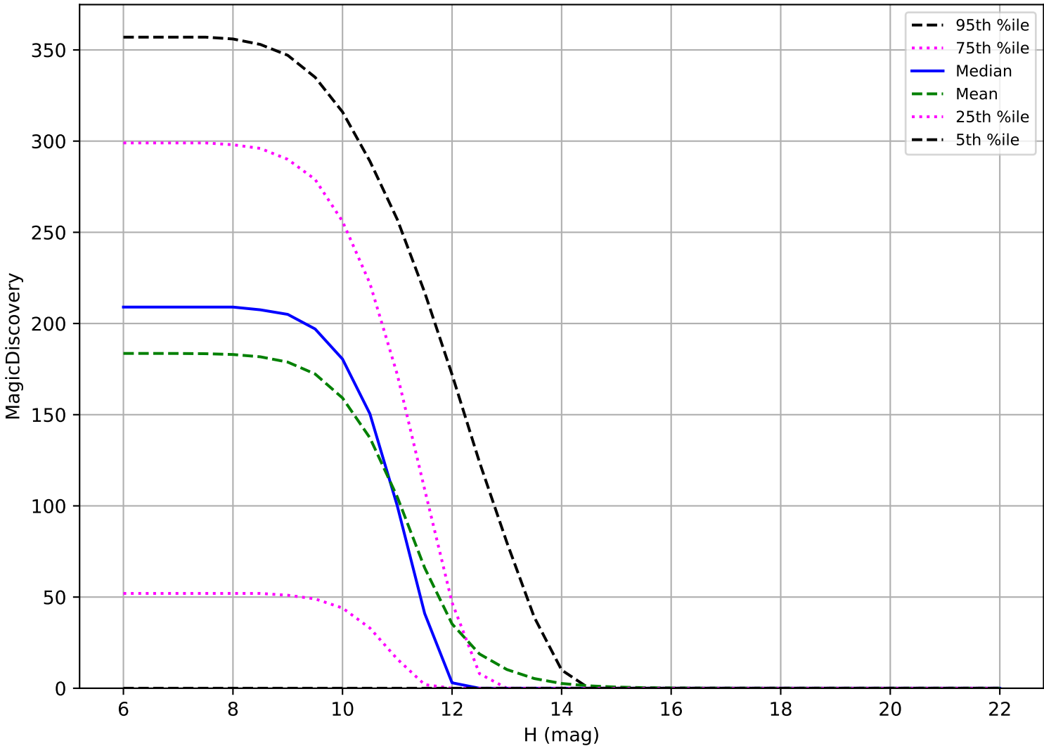
internal_u_expt27_nscale1.2v3.4_10yrs: OCC_r20 6 detections in 60 nights detection loss
