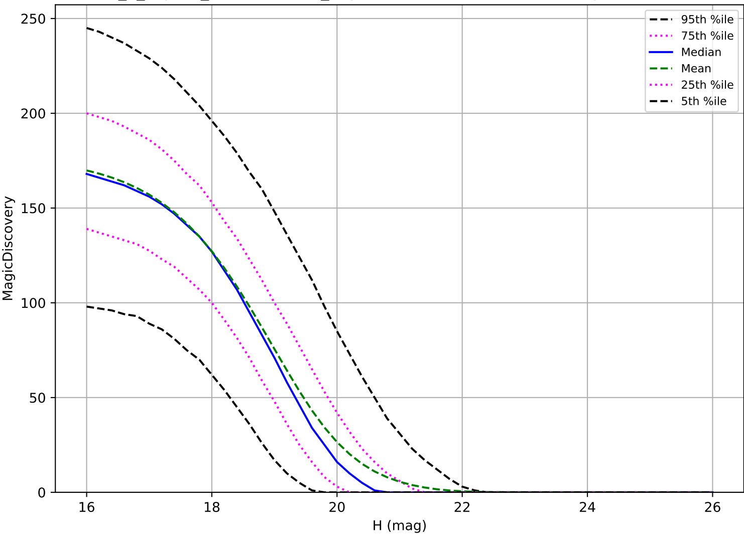
internal_u_expt27_nscale1.2v3.4_10yrs: MBA 6 detections in 60 nights detection loss
