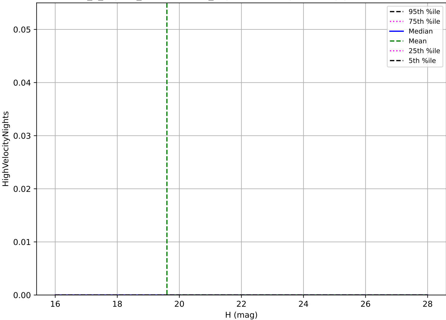
internal_u_expt27_nscale1.2v3.4_10yrs: Vatira High velocity pair detection loss
