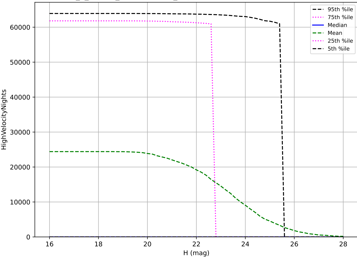
internal_u_expt27_nscale1.2v3.4_10yrs: PHA High velocity pair detection loss
