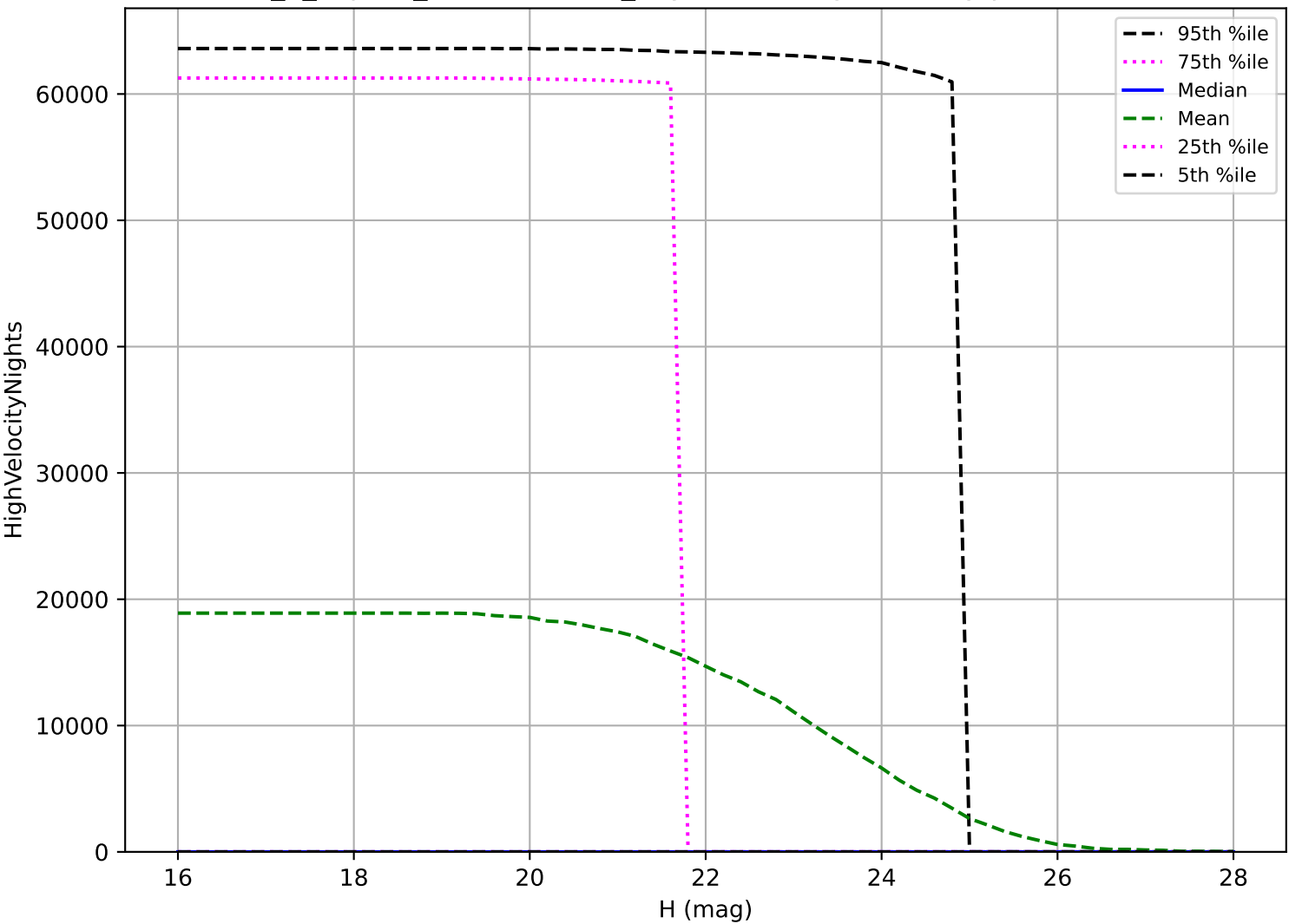
internal_u_expt27_nscale1.2v3.4_10yrs: NEO High velocity pair detection loss
