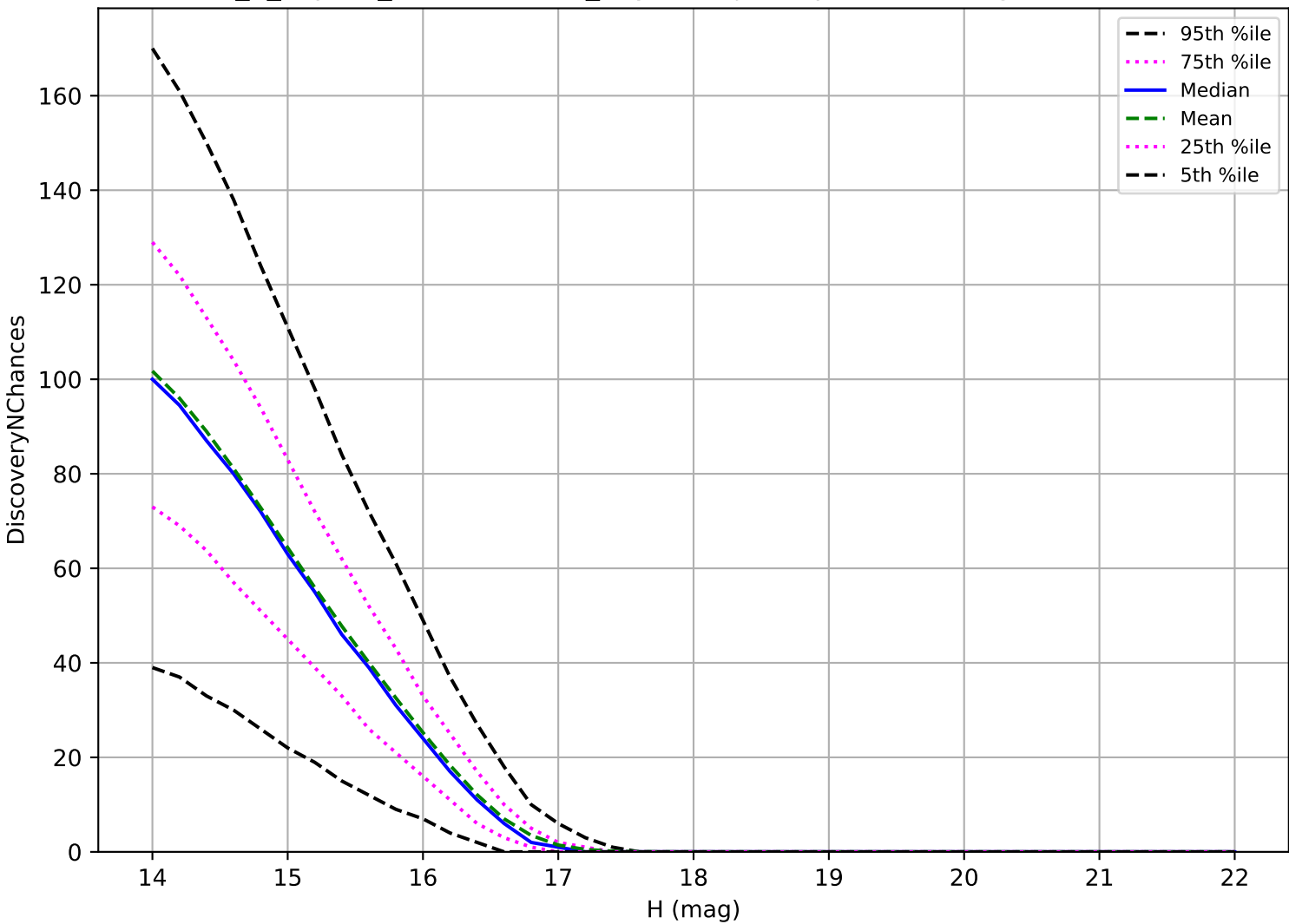
internal_u_expt27_nscale1.2v3.4_10yrs: Trojan 3 pairs in 15 nights detection loss
