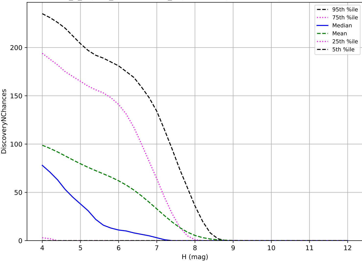
internal_u_expt27_nscale1.2v3.4_10yrs: TNO 3 pairs in 15 nights detection loss
