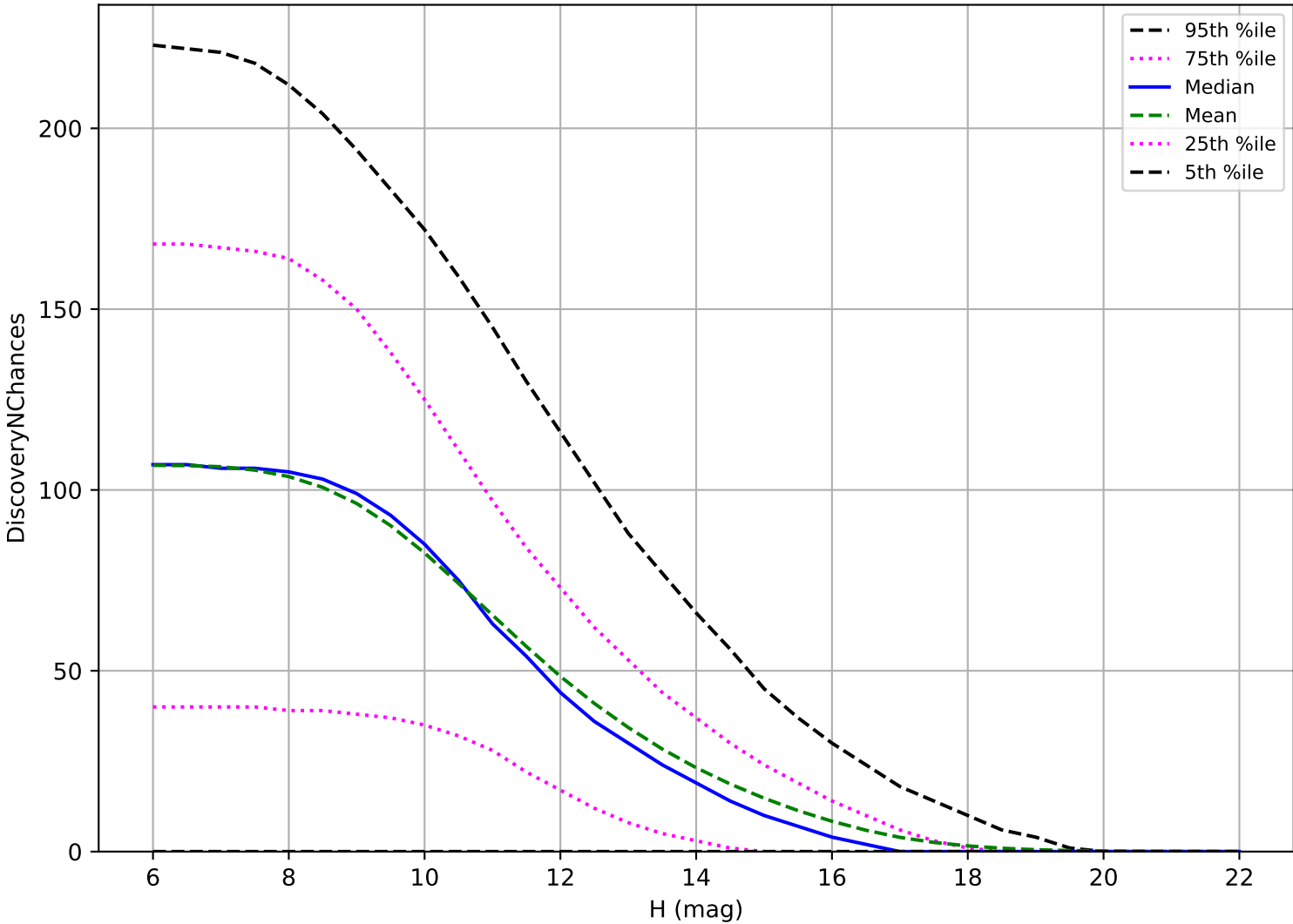
internal_u_expt27_nscale1.2v3.4_10yrs: OCC_r5 3 pairs in 15 nights detection loss
