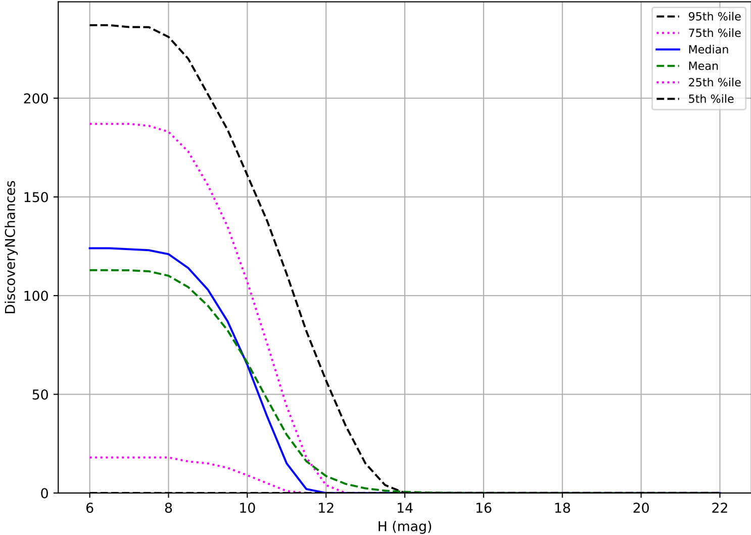
internal_u_expt27_nscale1.2v3.4_10yrs: OCC_r20 3 pairs in 15 nights detection loss
