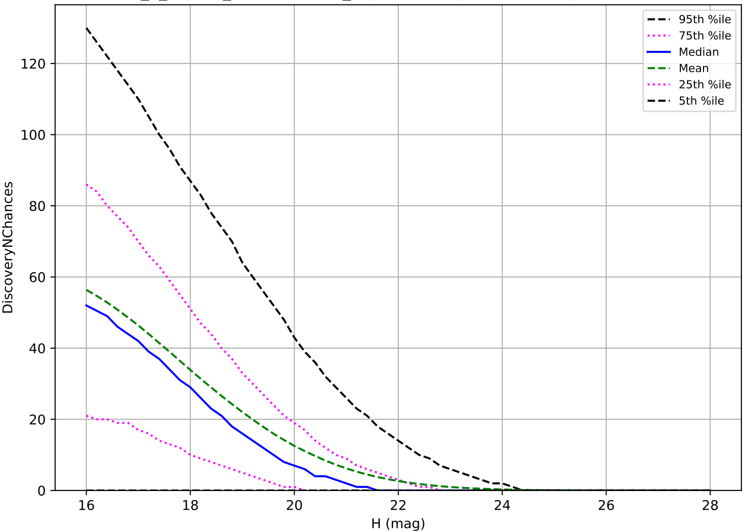
internal_u_expt27_nscale1.2v3.4_10yrs: NEO 3 pairs in 15 nights detection loss
