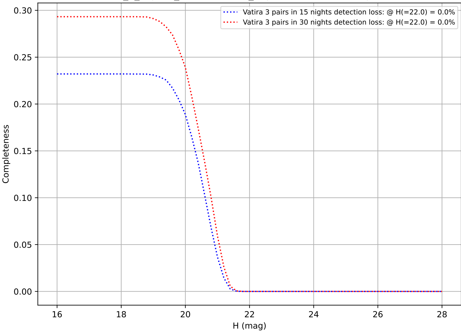
internal_u_expt27_nscale1.2v3.4_10yrs: DifferentialCompleteness
