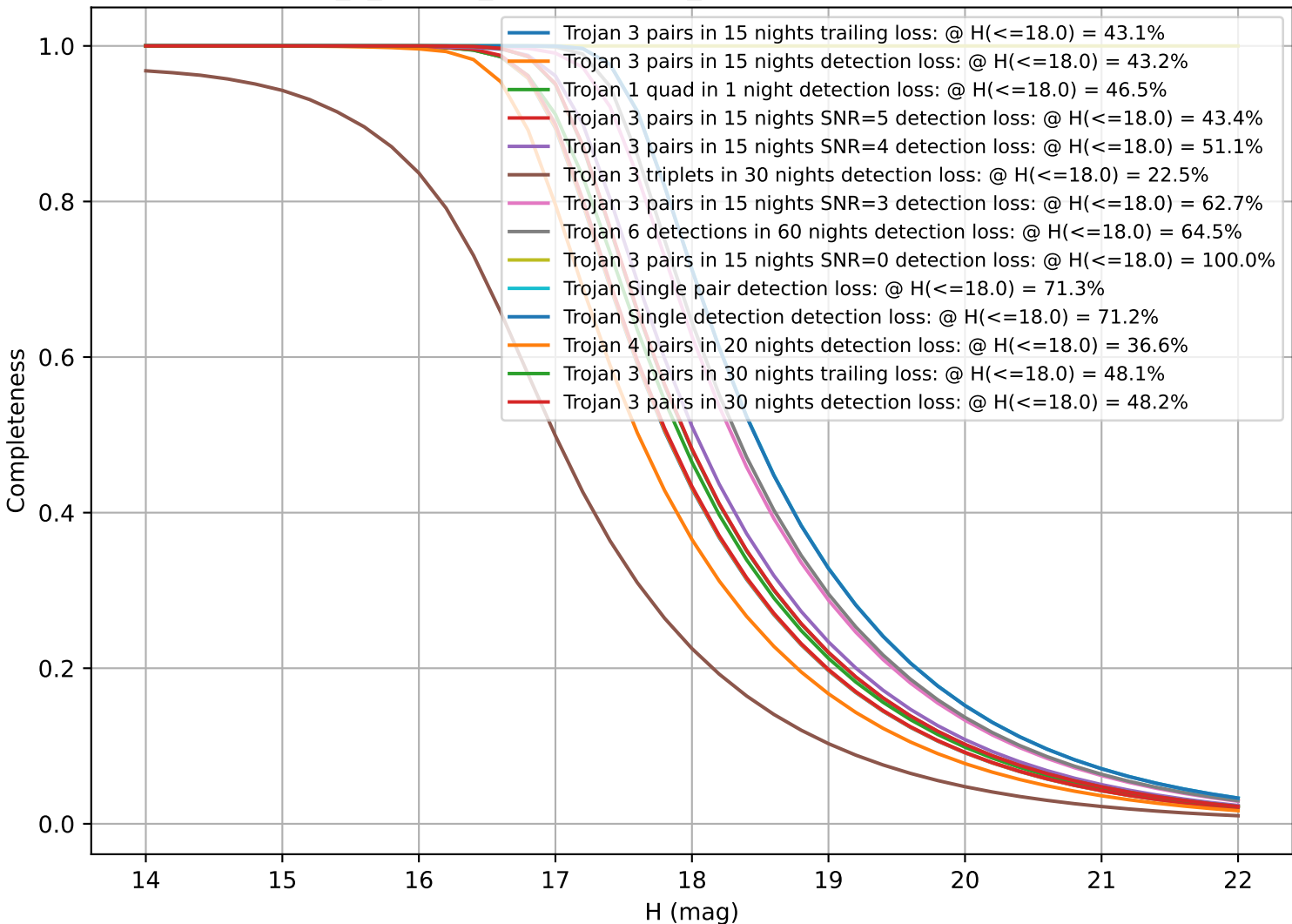
internal_u_expt27_nscale1.2v3.4_10yrs: CumulativeCompleteness
