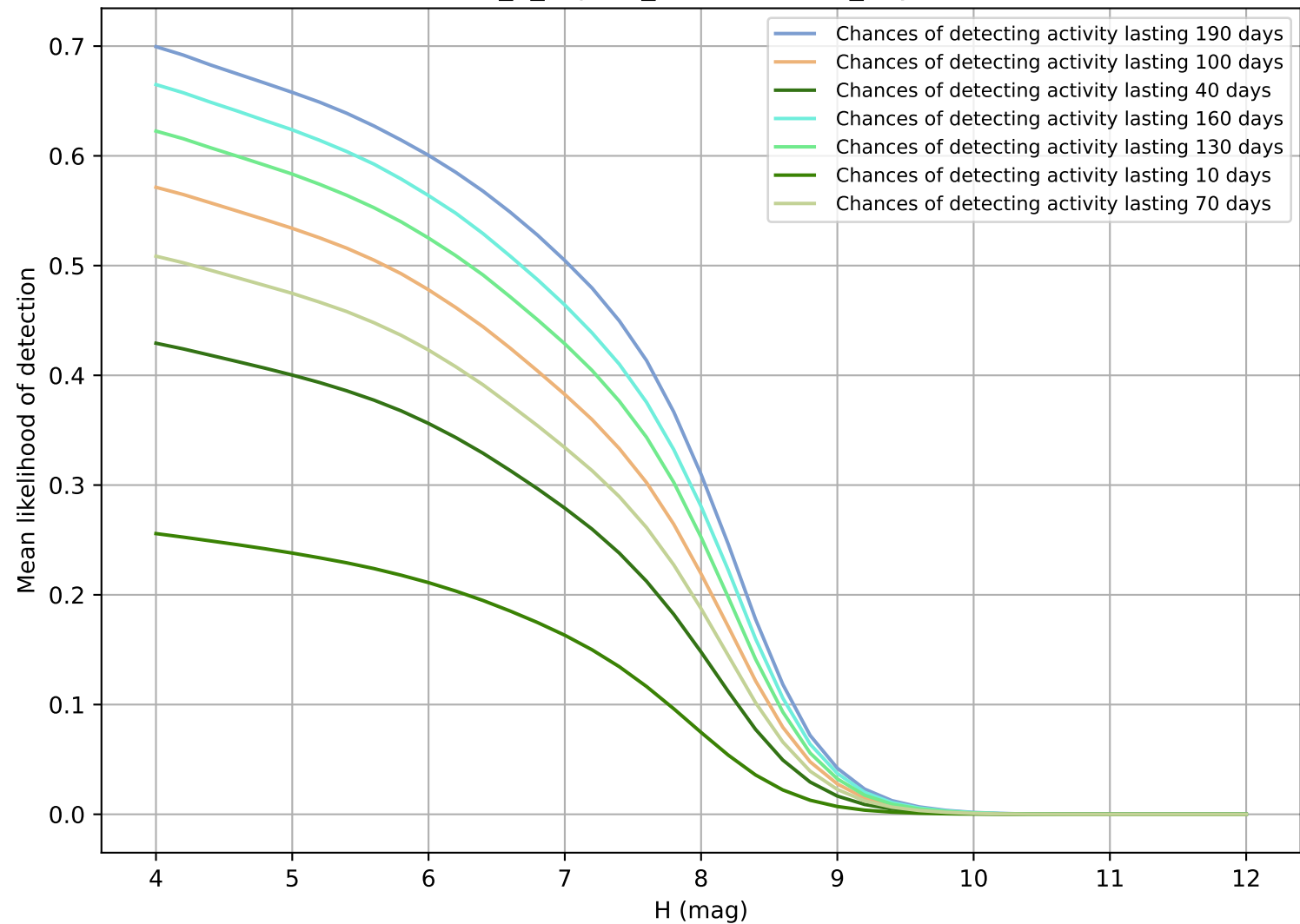
internal_u_expt27_nscale1.2v3.4_10yrs TNO
