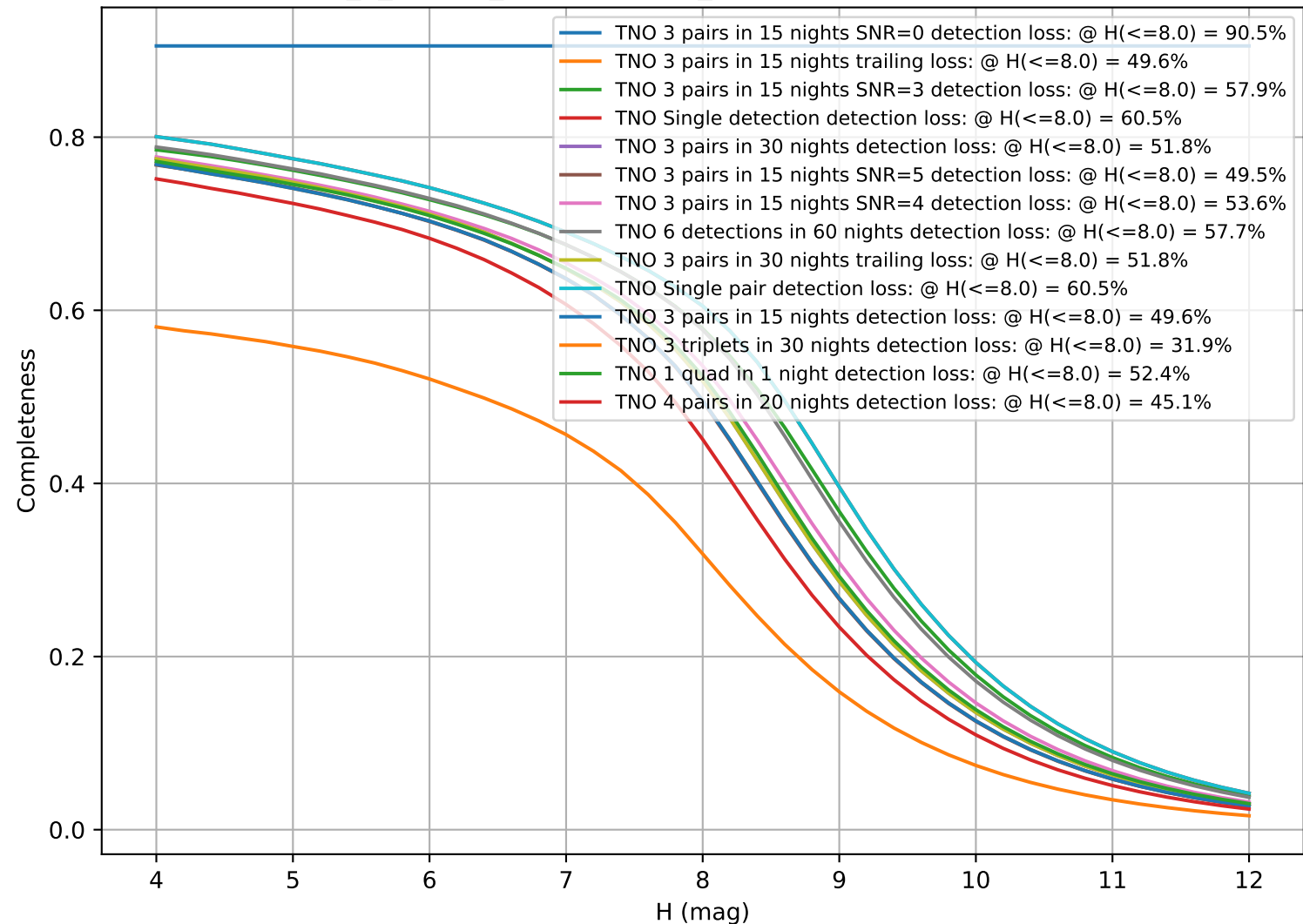
internal_u_expt27_nscale1.2v3.4_10yrs: CumulativeCompleteness
